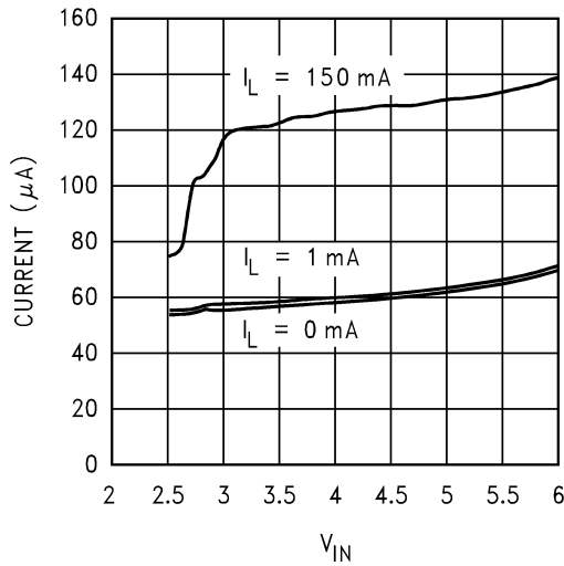
Ground Current vs V IN @ 25°C
