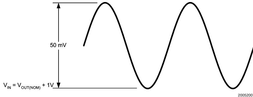
FIGURE 2. PSRR Input Test Signal
